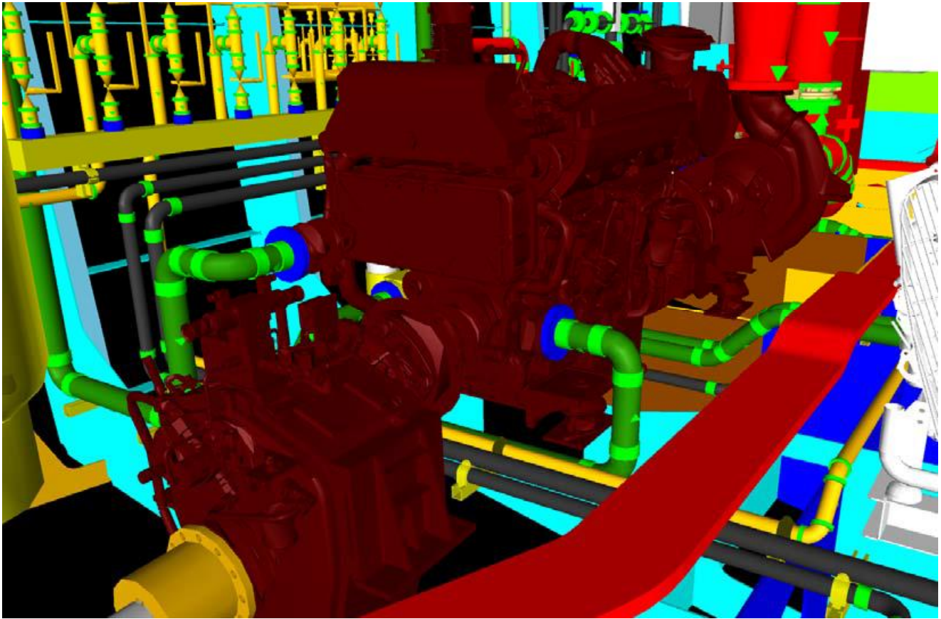
3D Model of Main Engine Room: Port Side Main Engine Shown
